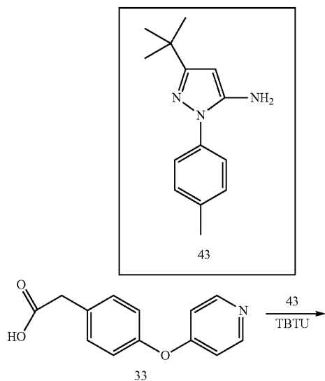
Scheme 9.
