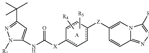
Formula V
