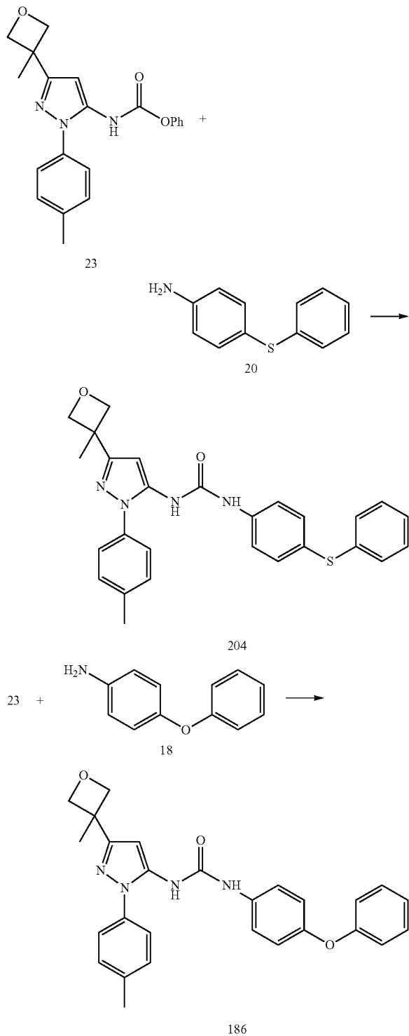
Scheme 6.
