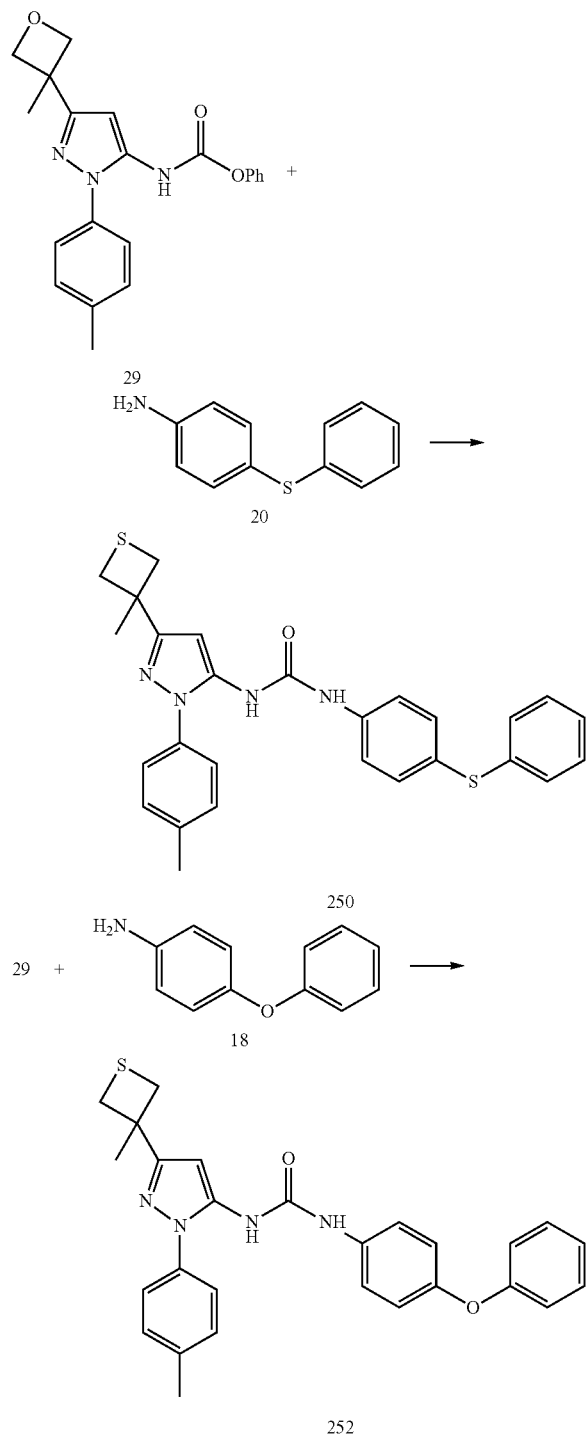
Scheme 7.
