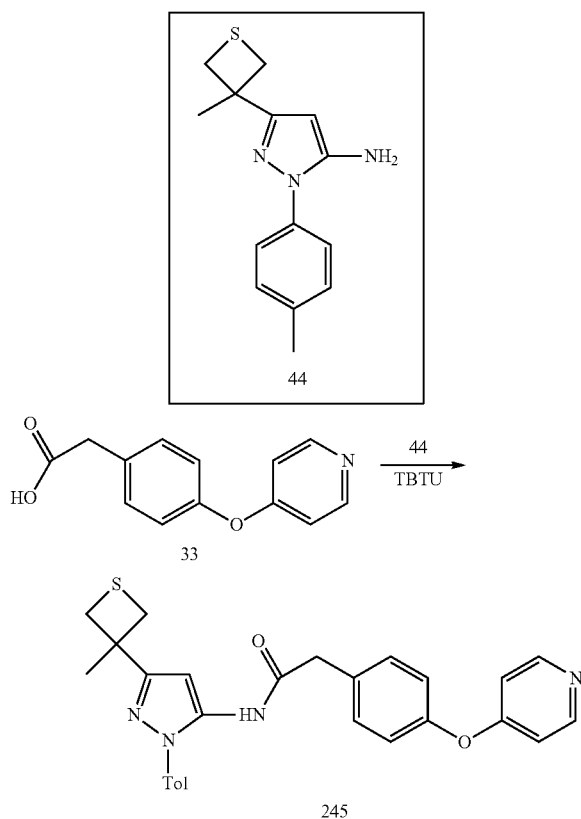
Scheme 10.
