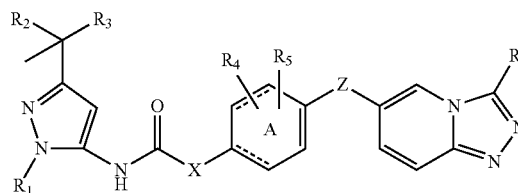
Formula IV
