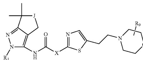
Formula VII
